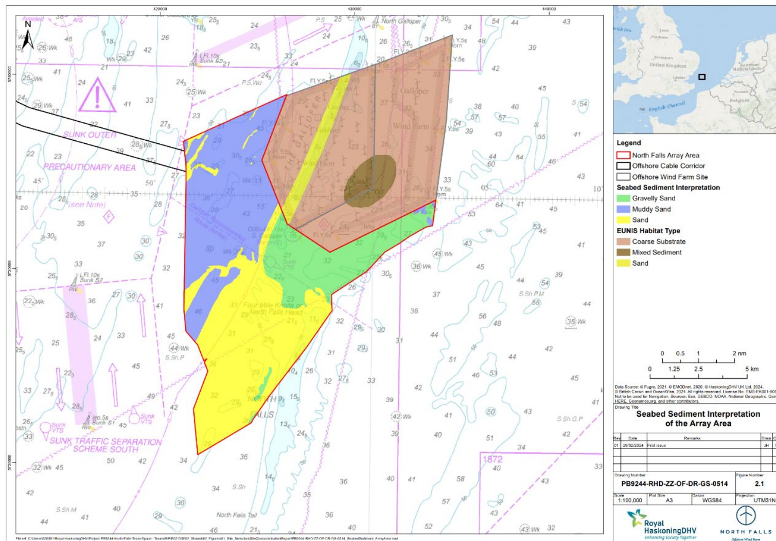
Figure 2.1 North Falls sediment distribution – array area
